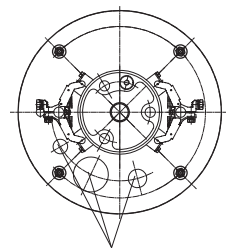
Bore holes in the floor panel intended for the following screw connections: 1x M50x1.5 1x M25x1.5 1x M20x1.5
