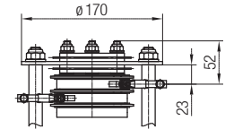
Version with support disk for 8 rings
