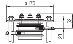
Version with support disk for 8 rings
