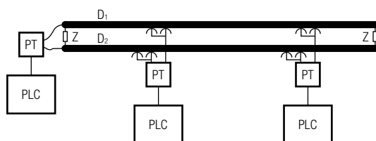
Straight arrangement with end feed
