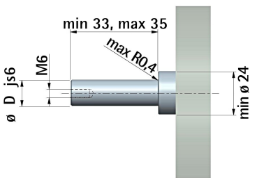
Optional shaft configurations available upon request
