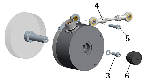
ZCU, ZCZ connections
