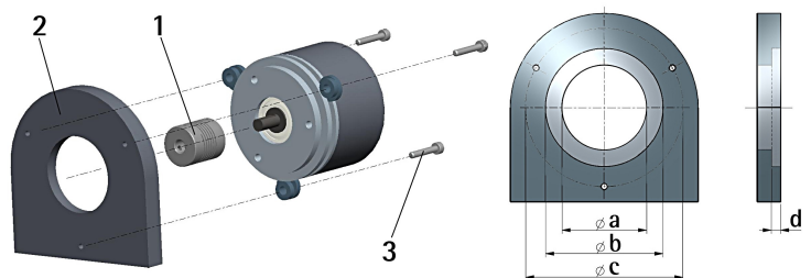
I58, I58S, I65, MI58, MI58S with fixing clamps
