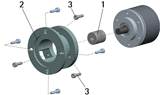
I58S, I65 with mounting bell
