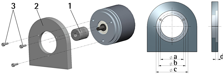
I58, I58S, I65, MI58, MI58S
