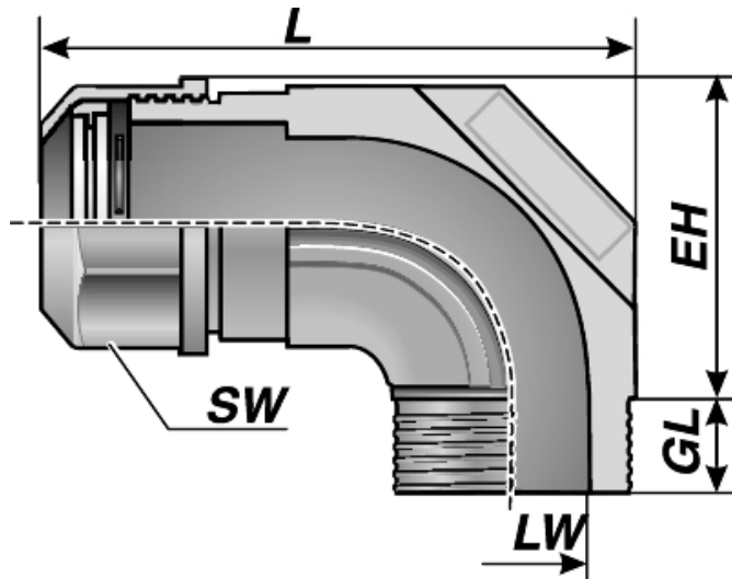
Dimensional drawing
