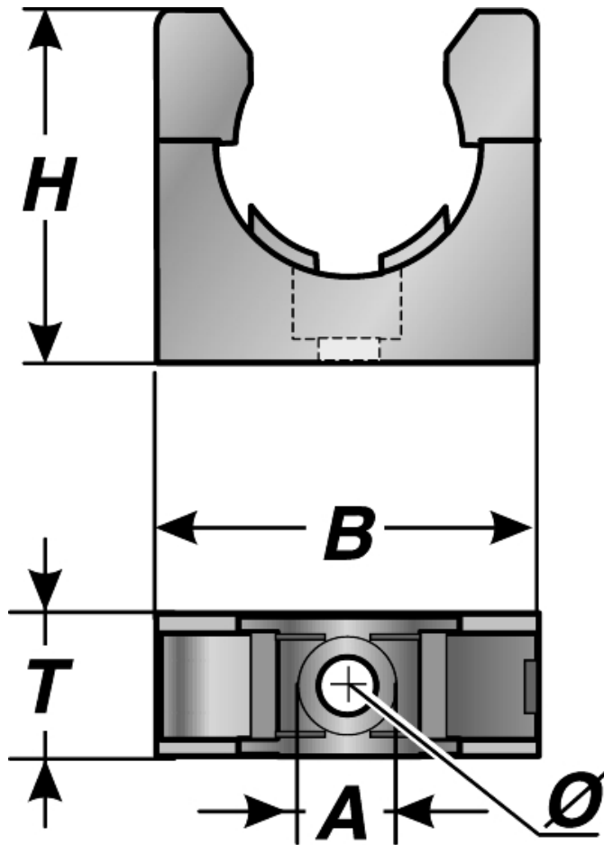
Dimensional drawing
